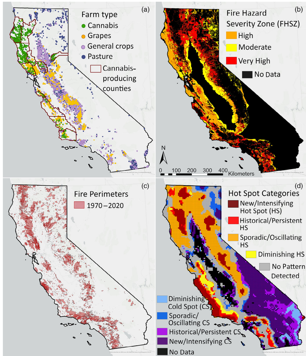
FIGURE 1 Study area map. (a) Farm types (cannabis, grapes, pasture, and general crops) and cannabis-producing counties (restricted to those comprising at least 1% of Department of Cannabis Control outdoor cannabis licenses). (b) Fire hazard severity zones, as established by the State of California (CAL FIRE). (c) Wildfire perimeters dating back 5 and 50 years. (d) Burn pattern projections from 2020 to 2100 as established by Moanga et al. (2020).
