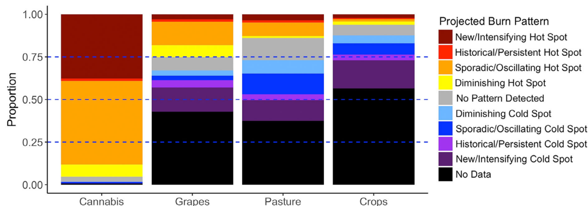
FIGURE 4 Projected burn regimes by agricultural type. Proportions of cultivation area of the four agricultural types within each projected burn pattern category are summarized. Categories are adapted from those used by Moanga et al. (2020). No data values result from areas for which burn probability data from Westerling (2018) were not produced due to extremely low likelihood of wildfire. Maps depicting projected burn patterns are available in Moanga et al. (2020).
