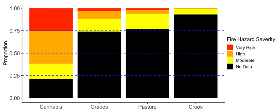
FIGURE 2 Fire hazard severity zones (FHSZs) by agricultural type. Proportions of farms of the four agricultural types within each FHSZ category are summarized, within cannabis-producing counties only. FHSZs are categorized as moderate, high, and very high, with no data values resulting from areas not categorized either due to a lack of fire danger or federal fire responsibility or local fire responsibility zones.
