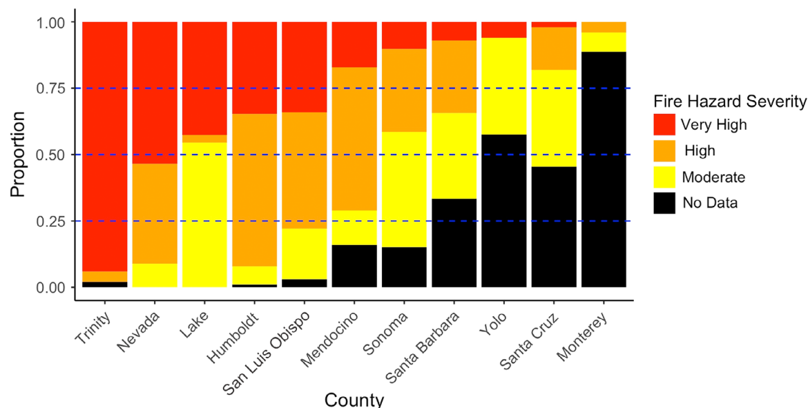
FIGURE 5 Fire hazard severity zones (FHSZs) by county. Proportions of cannabis cultivation within each FHSZ category are summarized by county. FHSZs are categorized as moderate, high, and very high, with no data values resulting from areas not categorized either due to a lack of fire danger or federal fire responsibility or local fire responsibility zones.
