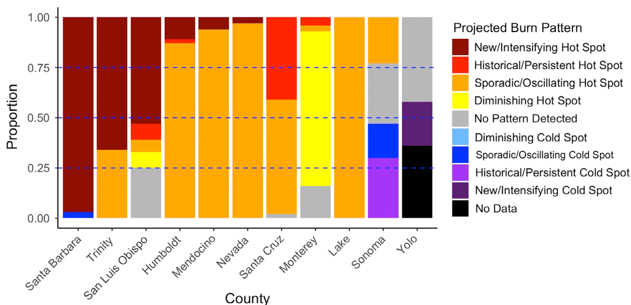
FIGURE 6 Projected burn regimes by county for cannabis agriculture. Proportions of cannabis cultivation within each projected burn pattern category are summarized by county. Categories are adapted from those used by Moanga et al. (2020). No data values result from areas for which burn probability data from Westerling (2018) were not produced due to extremely low likelihood of wildfire. Maps depicting projected burn patterns are available in Moanga et al. (2020).
