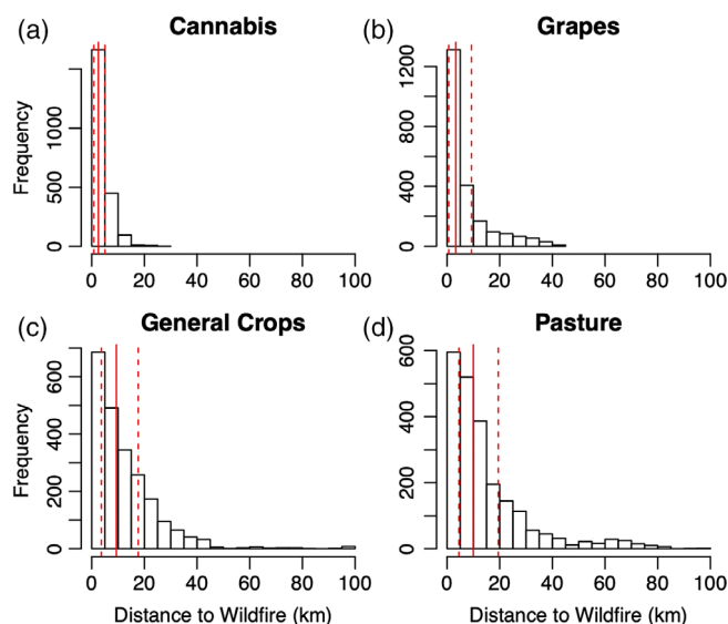
FIGURE 3 Farm proximities to known wildfires. Perimeters for fires since 1970 are compared against the geospatial locations of (a) cannabis and sampled locations for (b) grapes, (c) general crops, and (d) pasture. Median values for each agricultural type are indicated by a solid red line, with the interquartile range represented with dashed red lines.
